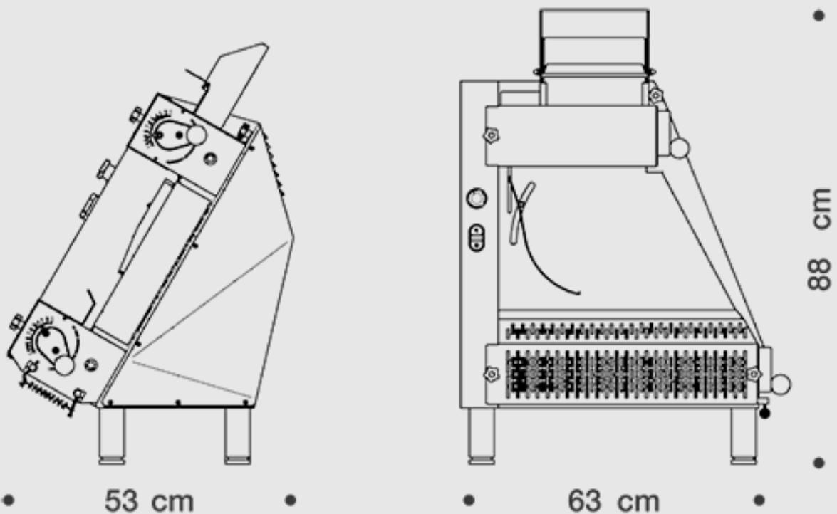
M51: Heavy-duty dough sheeter
